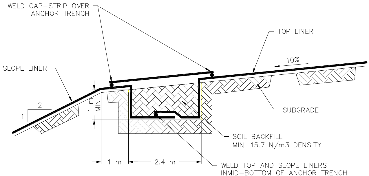
Figure 2. Typical Anchor Construction Detail.
