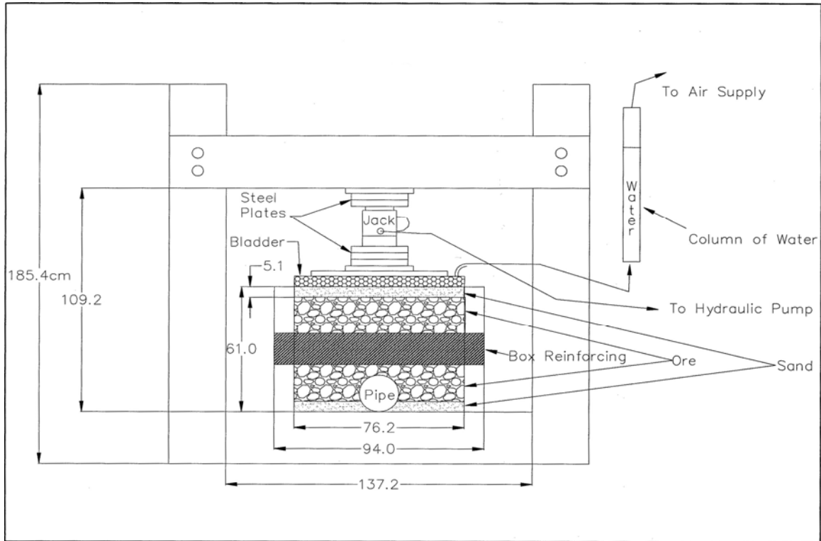
Figure 1 - Test Apparatus
