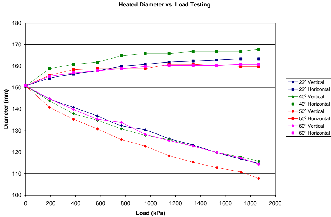
Figure 2 - Pipe Loadings and Varying Temperatures
