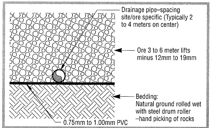
Figure 2. Leach pad liner system
