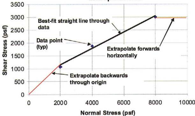
Figure 4 | Example of safe shear strength extrapolation.
